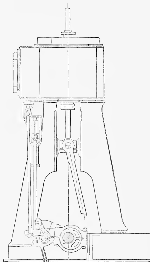
Marshall's Patent Valve Gear.
